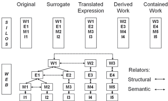
DIAGRAM 4. Metadata silos vs web of links
