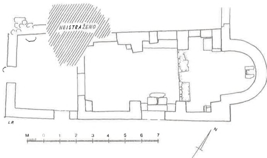
Sl. 5. Tloris ostataka Crkve Sv. Ivana u Telašćici kod Sali (I. Petricioli). Fig. 5. The ground-plan of the remains of St John's church in Telašćica near Sali (I. Petricioli).
